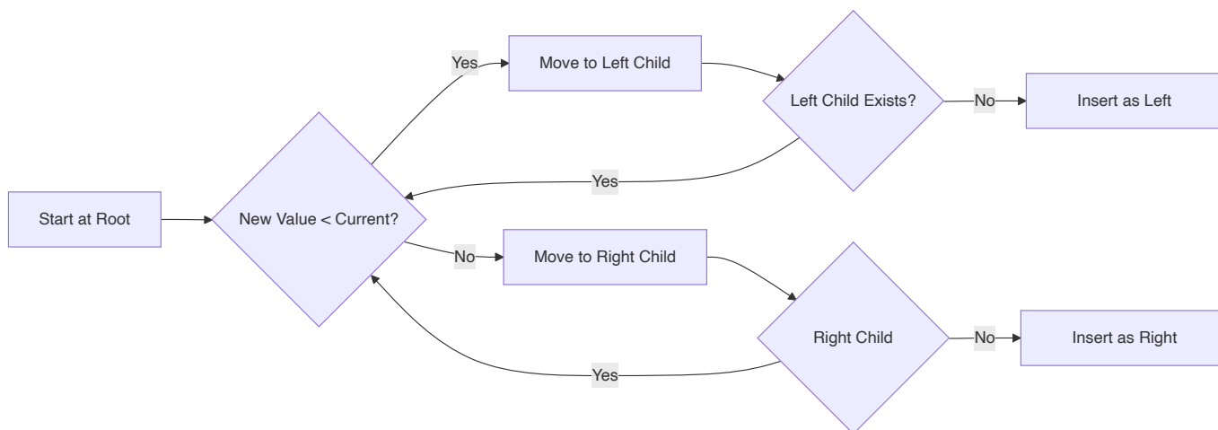
Diagram: BST Insertion
